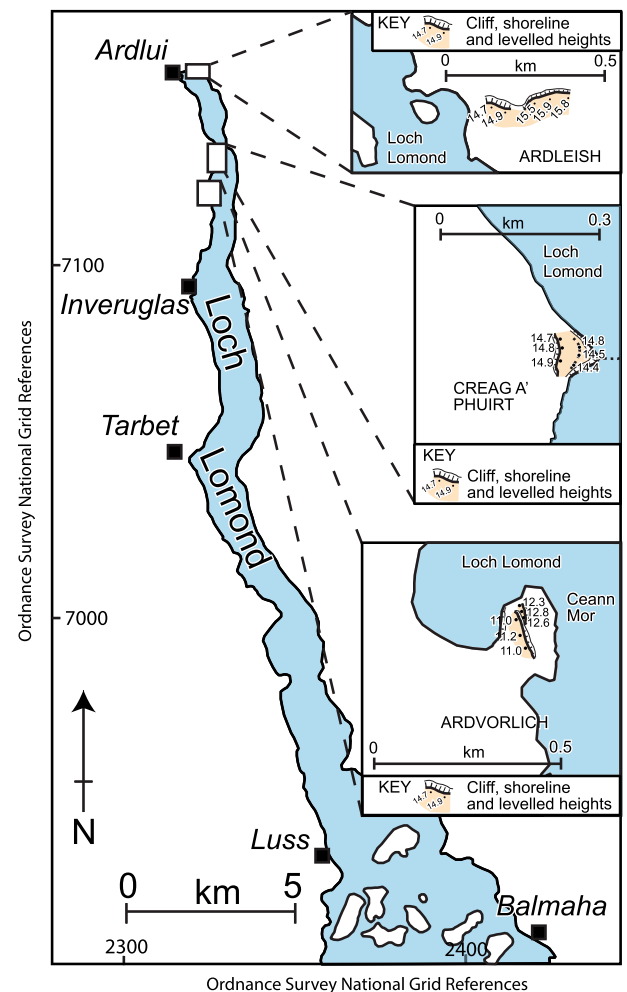
Fig. 3. Northern Loch Lomond shoreline fragments.
