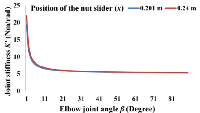
Figure 15. Elbow joint stiffness with nut slider position
