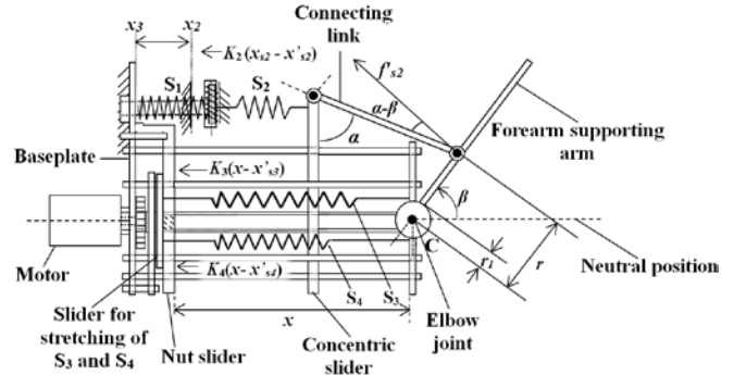
Figure 14. Generation of resistive force in the exoskeleton
