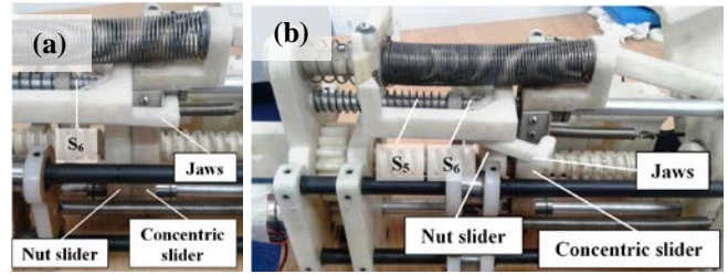
Figure 4. Switching from motor controlled to assistive mode
