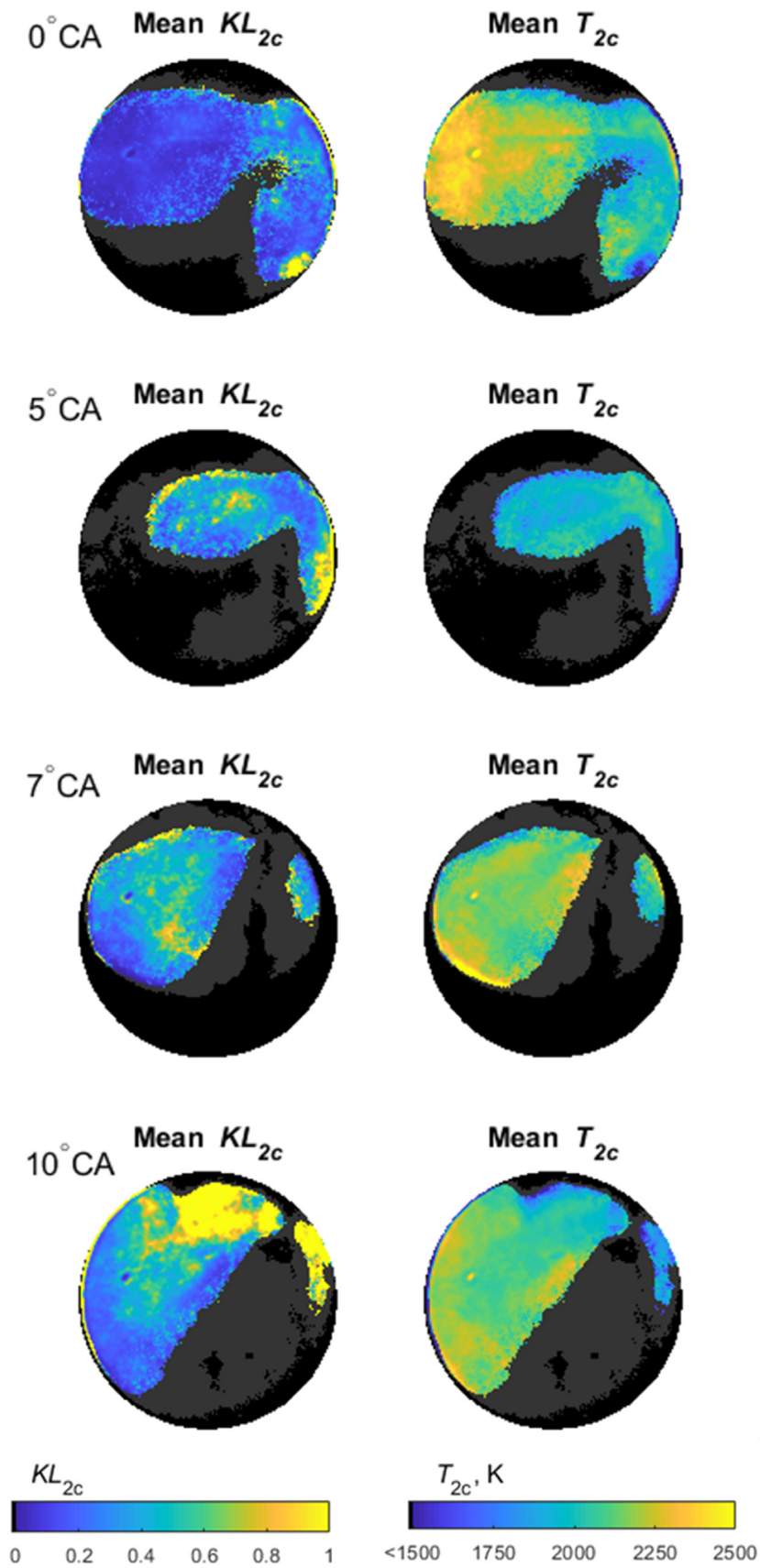
Fig. 10. Ensemble-averaged T_{2c} and KL_{2c} images at 0^\circ CA, 5^\circ CA, 7^\circ CA and 10^\circ CA ATDC, from 50 cycles - the grey regions represent regions excluded from visualization as described in the text.
