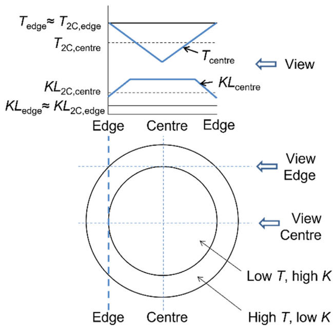
Fig. 14. Idealized developed flame (at 10 °CA ATDC) soot KL and temperature distribution and flame cross section, showing relationship between edge and centreline measurements and edge and centreline real distributions.
