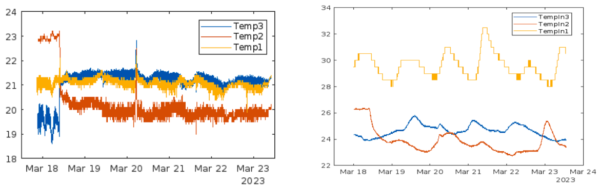
Fig. 21. Data graphs showing comparisons of temperature values (a) in farm and (b) inside bags.
