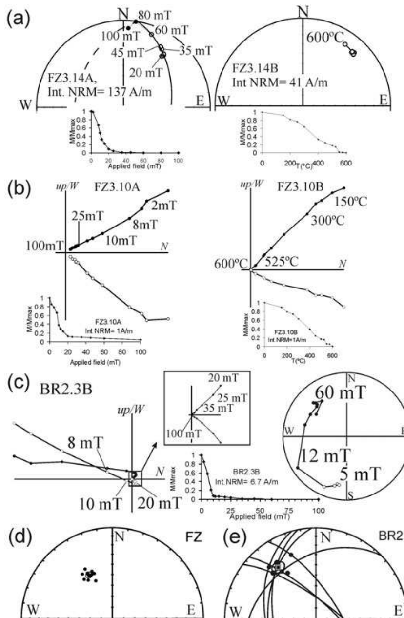
Figure 5. Orthogonal vector diagrams, equal area projections and normalized magnetization decays during AF and TH demagnetization of typical FZ dyke samples. (a) Rejected specimens (from the same sample, FZ3.14) exhibiting anomalously strong NRM due to lightning strikes. (b) Accepted specimens (the same sample, FZ3.10) with one stable component. (c) Accepted specimen (BR2.3B) with two overlapping components. Equal area projection of specimen and site-mean directions for (d) single component (FZ) and (e) two overlapped components (BR2).
