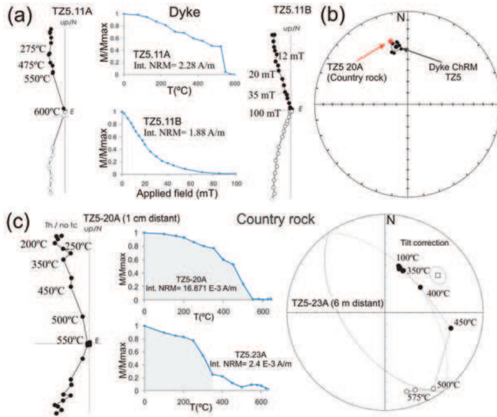
Figure 6. (a) Orthogonal vector diagrams and normalized magnetization decays during AF and TH demagnetization of typical IG dyke specimens (from the same sample, TZ5.11). (b) Equal area projection of specimen and site-mean directions for TZ5 IG site, including the mimic direction of the country rock sample TZ5.20 (without tilt correction). (c) Thermal demagnetization of country rock samples (TZ5.20 and TZ5.23; 1 cm and 6 m distant from the dyke margin, respectively). At increasingly distances from the IG dyke, country rocks show lower intensity NRM values and lower temperature partial thermoremanence phases (shaded area below the normalized magnetization decay); and a high unblocking temperature magnetic phase of reversed polarity, considered a pre-folding country rock ChRc, is observed.
