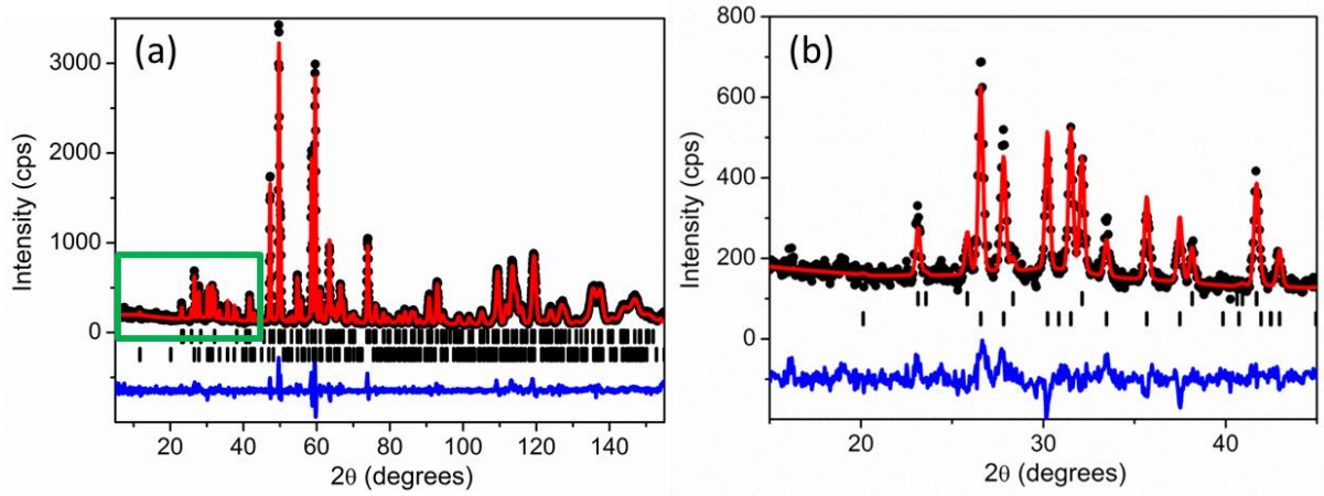
Figure 5: (a) Rietveld refinement of neutron diffraction data collected for \text{Ca}_2\text{Mn}_3\text{O}_8 at 4 K. Where the black circles are the observed data, the red line is the calculated model and the blue line is the difference curve. The bottom tick marks are the C2/m phase and the top tick marks represent the magnetic Bragg reflections. (b) Shows a zoomed in region at high d -spacing (as shown in the box in figure (a)) showing the magnetic Bragg peaks more clearly. (Colour online)
