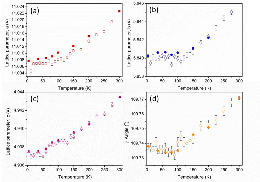
Figure 4: Lattice parameters (a) a, (b) b, (c) c, and (d) \beta angle as a function of temperature showing a invariant effect in the lattice b-direction and \beta angle which persists up to a temperature of approximately 130 K. Open and closed symbols are XRD and neutron diffraction data respectively. Note: error bars indicate 1 standard deviation and in some data are smaller than the symbol size.
