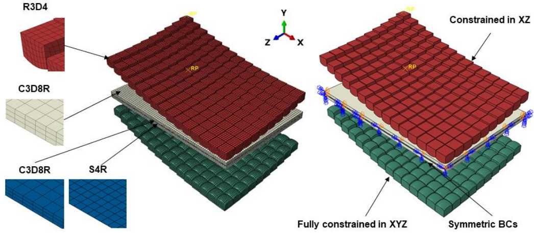
Figure 4: Schematic of the initial FE model, including element type and boundary conditions (BCs).
