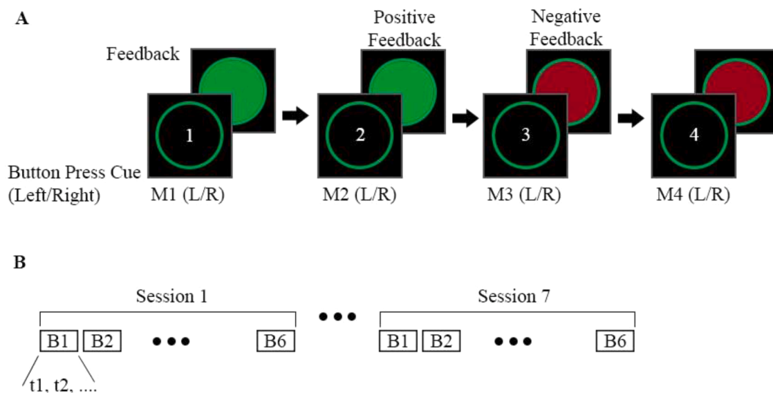
Fig. 2. Sequential stochastic learning task (A) Participants executed a sequence of four button presses (M1, M2, M3, and M4) using combinations of left and right button presses. At the start of each trial, participants were presented with an outline circle with a number as a cue to perform a button press. After each button press, they were given feedback about whether or not they were correct and were informed that 15% of the feedback will be misleading (B) Participants completed six sequences during each session (B1, B2, ..., B6) within which they responded to each trial ( t_1, t_2, \dots ). Participants had to learn and then execute the sequence correctly four times, at least two consecutive, before advancing to the next sequence in the set.
